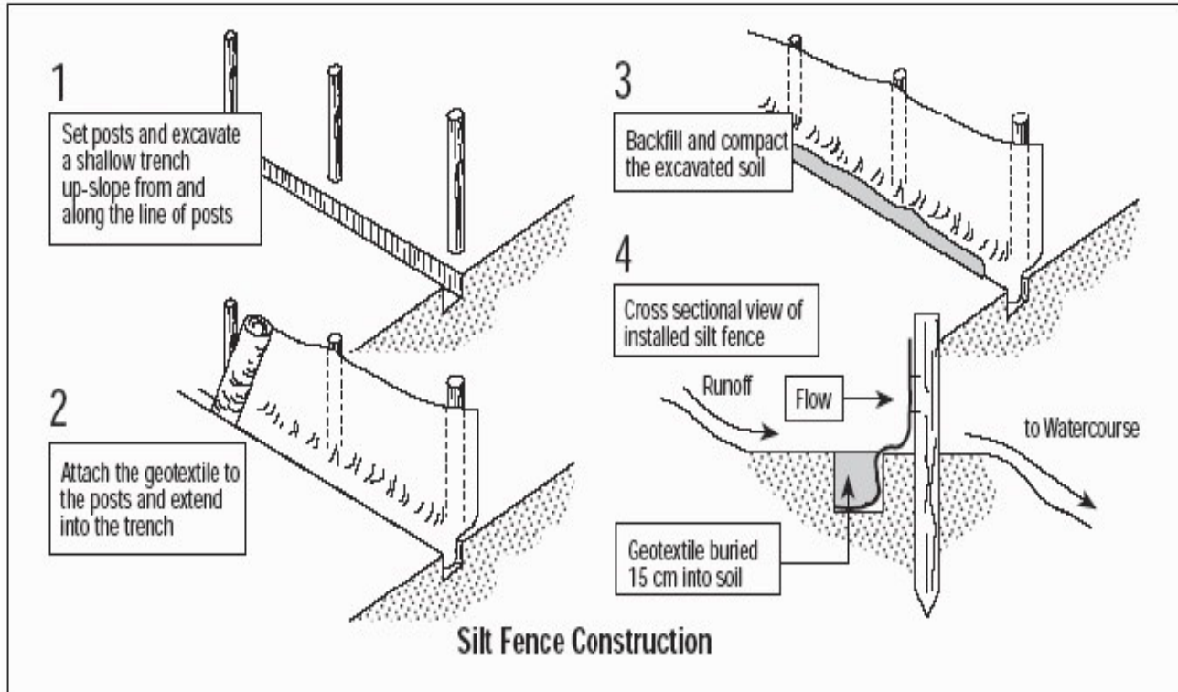
Figure 4 – Silt Fence Construction
