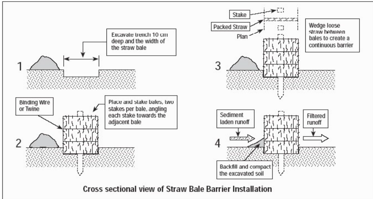
Figure 5 Straw/Hay Bale Barrier
